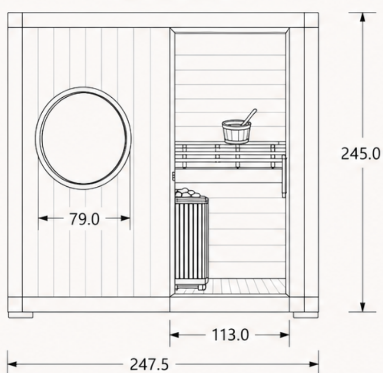
VISTA FRONTAL
